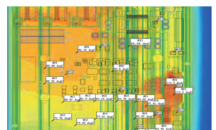
Thermal simulation
